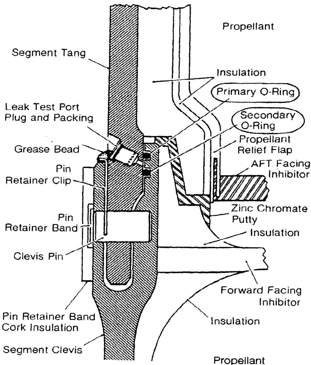
FIGURE 13. An incorrectly sealed leak test port could provide an escape route for a flame which burns past the primary O-ring.
