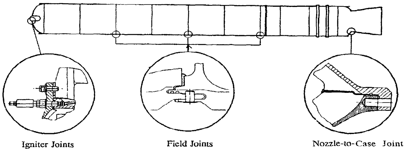
FIGURE 2. Locations and close-up views of booster-rocket field joints.
