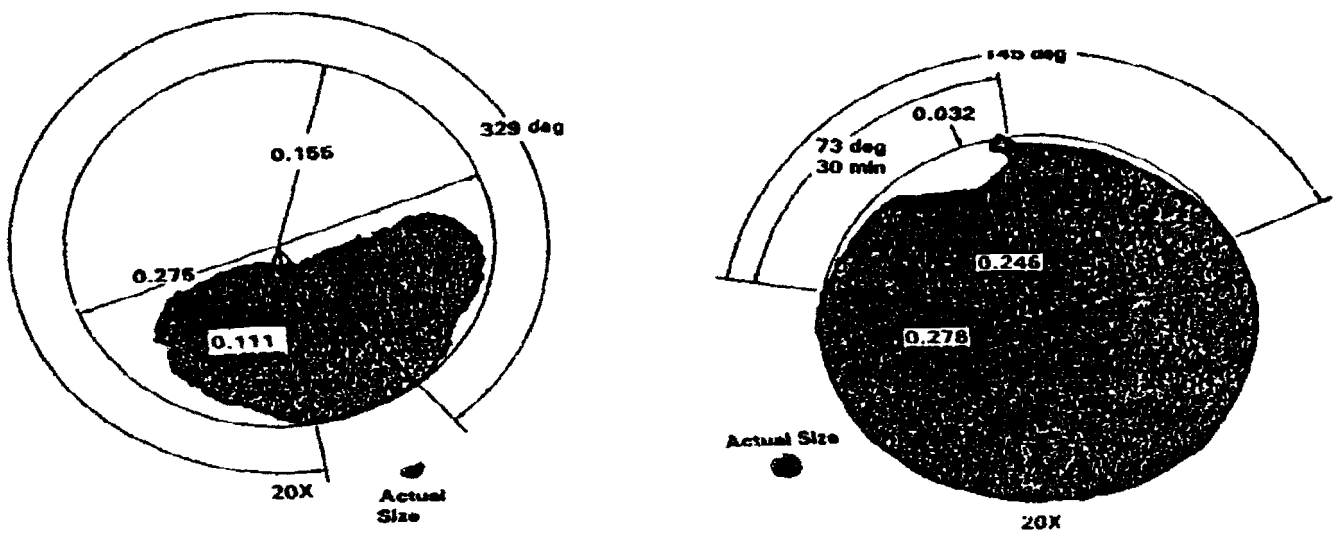
FIGURE 9. Two examples of O-ring erosion. Such erosion would occur unpredictably along 2 or 3 inches of the 37-foot O-ring.
