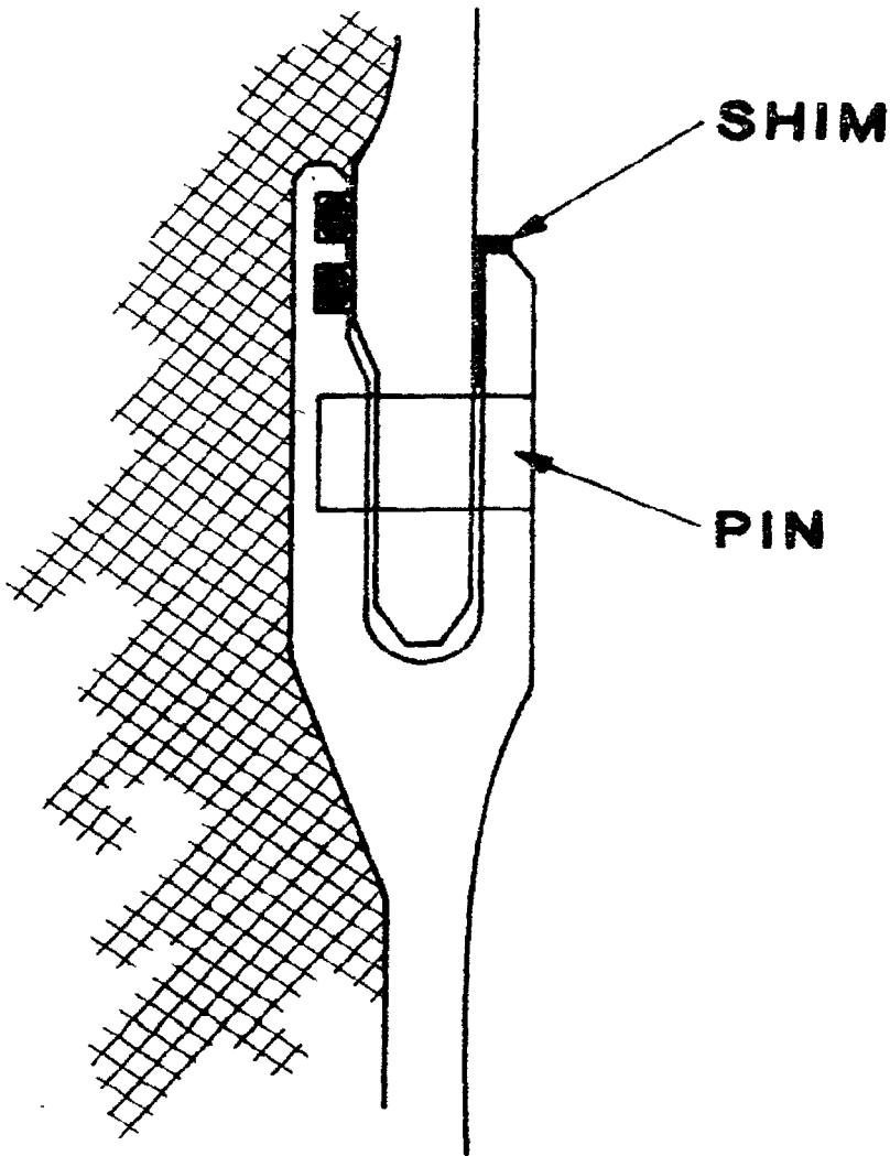
FIGURE 8. Thiokol attempted to cure the joint-rotation problem with shims.
