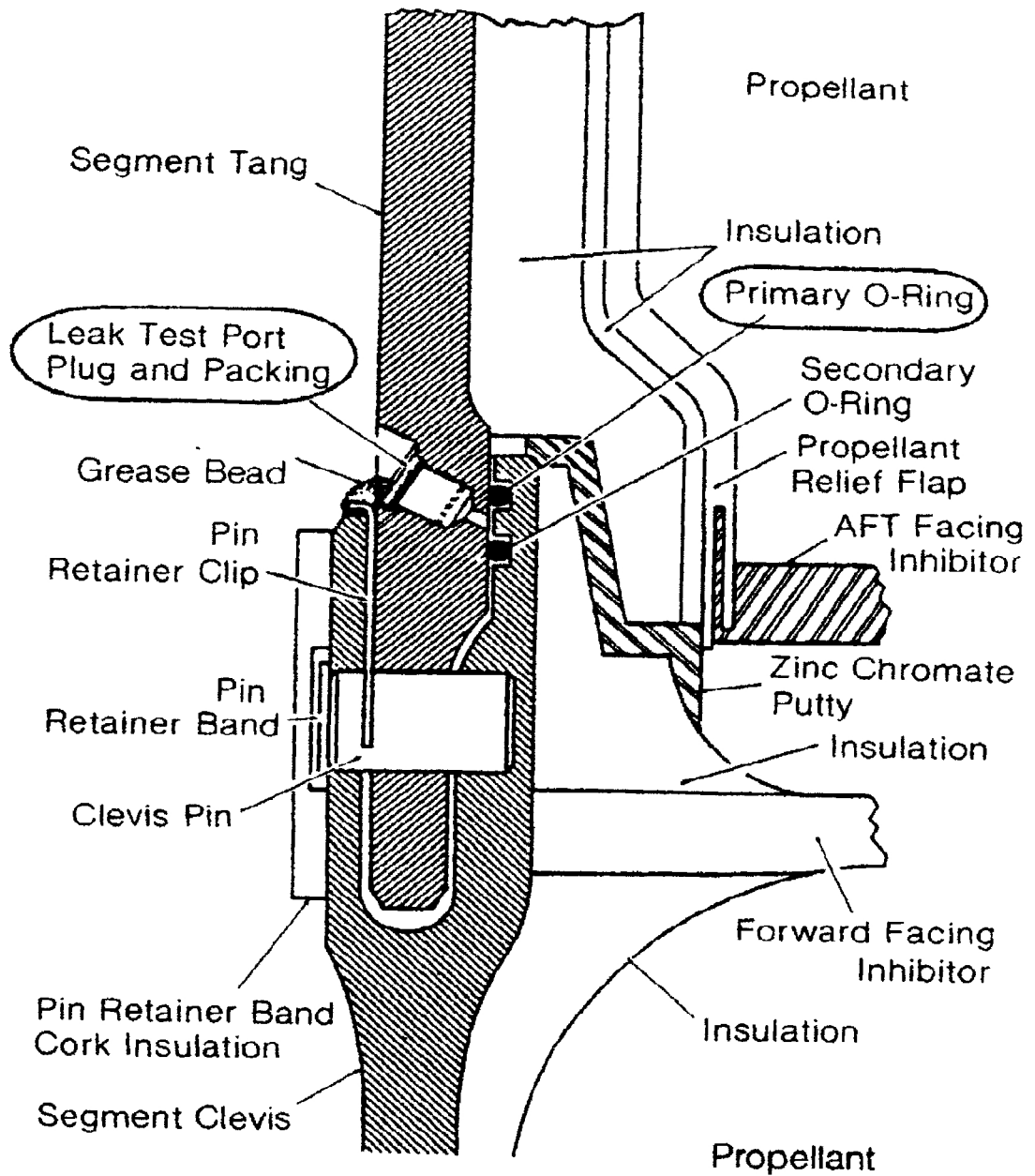
FIGURE 4. Detailed diagram of a field joint.
