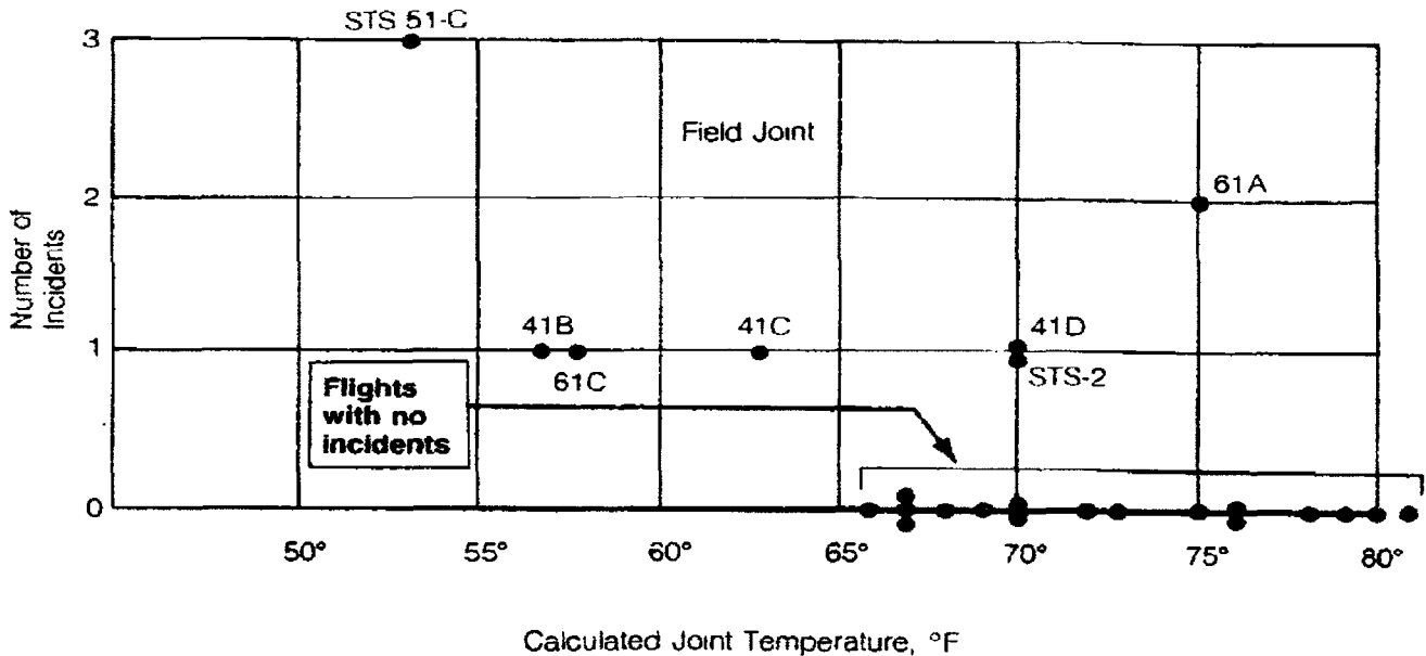
FIGURE 10. The correlation between temperature and O-ring incidents.
