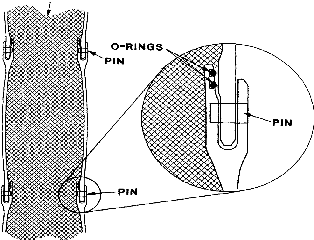
FIGURE 7. Joint rotation is caused by pressure from inside the rocket pushing the walls out farther than the joints. A gap opens, and hot gas flows past one or both of the O-rings.
